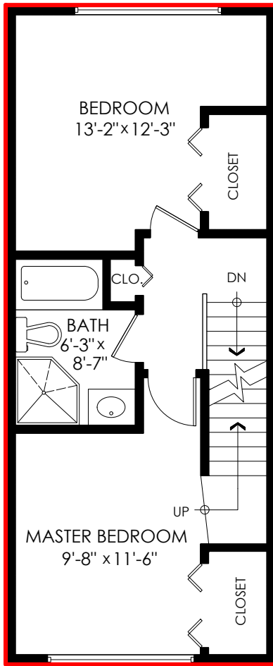
Upper Floor Plan Floor Area: 485 sq.ft. Ceiling Height: 8'
