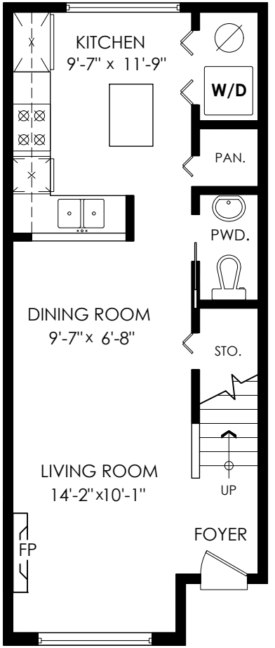
Main Floor Plan Floor Area: 468 sq.ft. Ceiling Height: 8'
