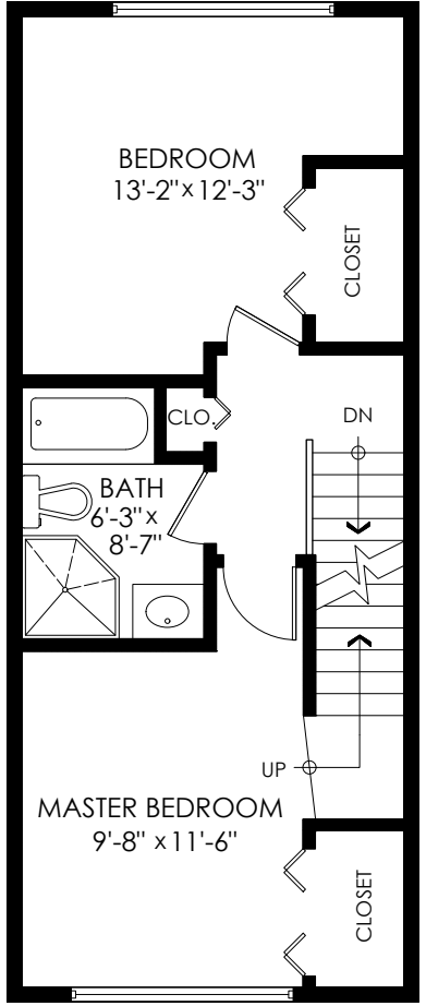
Upper Floor Plan Floor Area: 485 sq.ft. Ceiling Height: 8'
