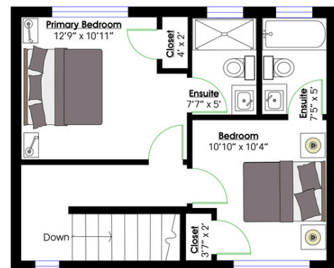
UPPER LEVEL LANEWAY Floor Area: 508 Sq. Ft. Ceiling Height: 8'1"
